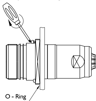
Vorderwandmontage front panel mounting
